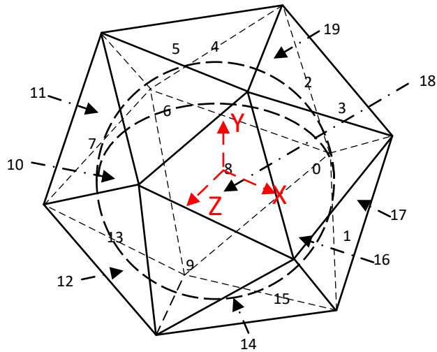
Figure 8. Icosahedron format
