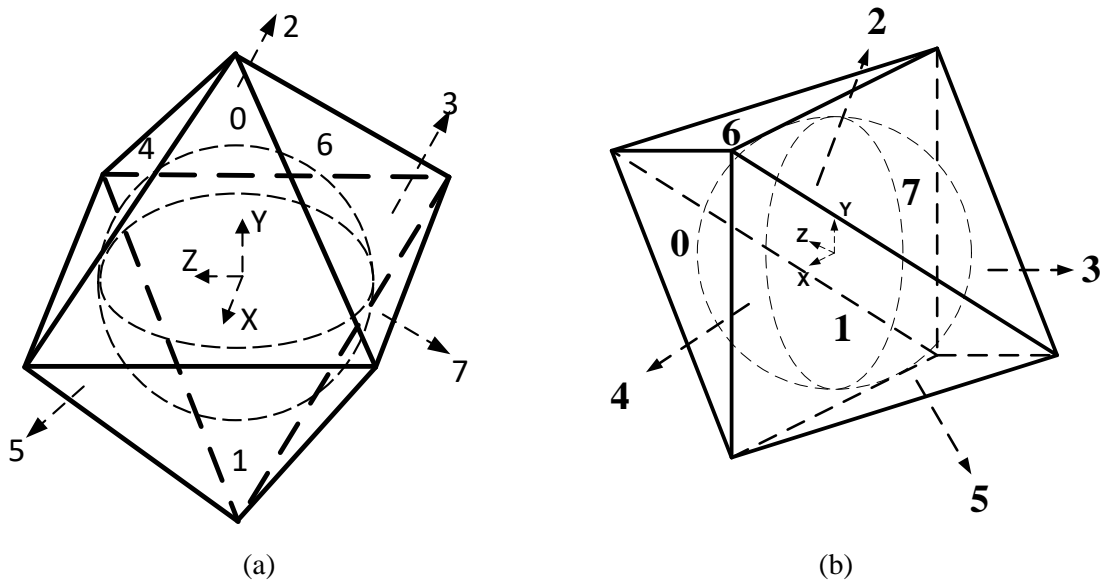
Figure 5. Octahedron definition: (a) definition for non-compact format; (b) definition for compact format
