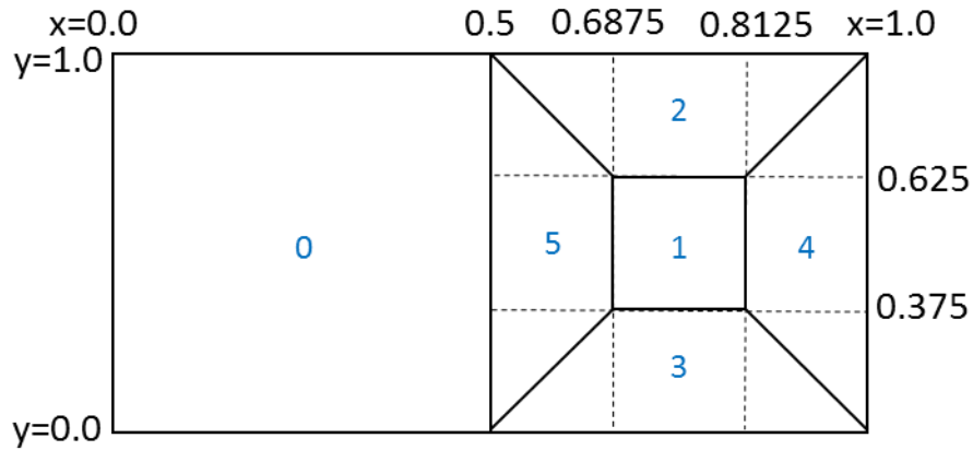
Figure 10. Truncated-square-pyramid frame packing format
