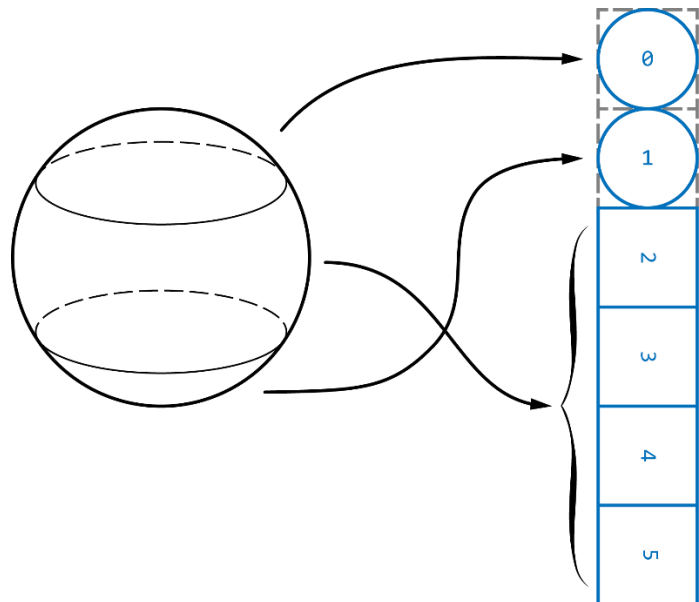
Figure 12. Segmented sphere conversion from sphere with vertical frame packing
