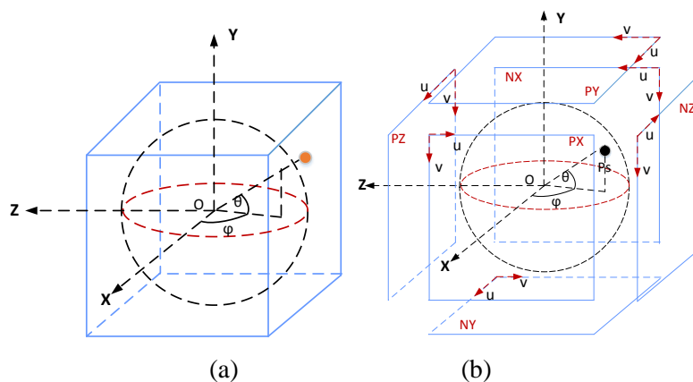
Figure 1. Cubemap format
