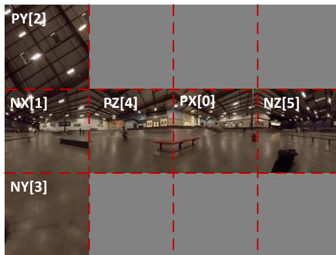
Figure 3. Cubemap 4x3 frame packing for the output: red dotted line indicates face boundary
