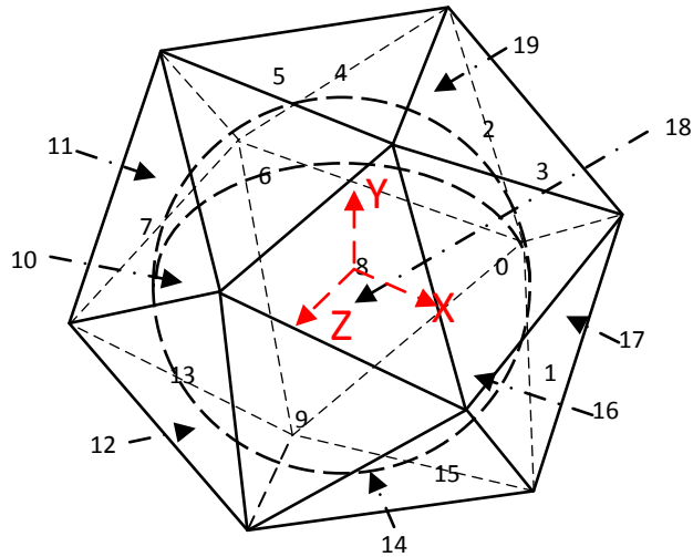
Figure 7. Icosahedron format
