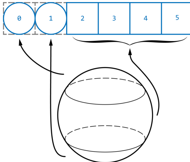
Figure 10. Segmented sphere conversion from sphere with horizontal frame packing
