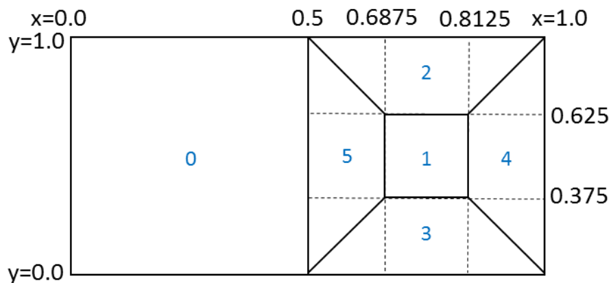
Figure 9. Truncated-square-pyramid frame packing format
